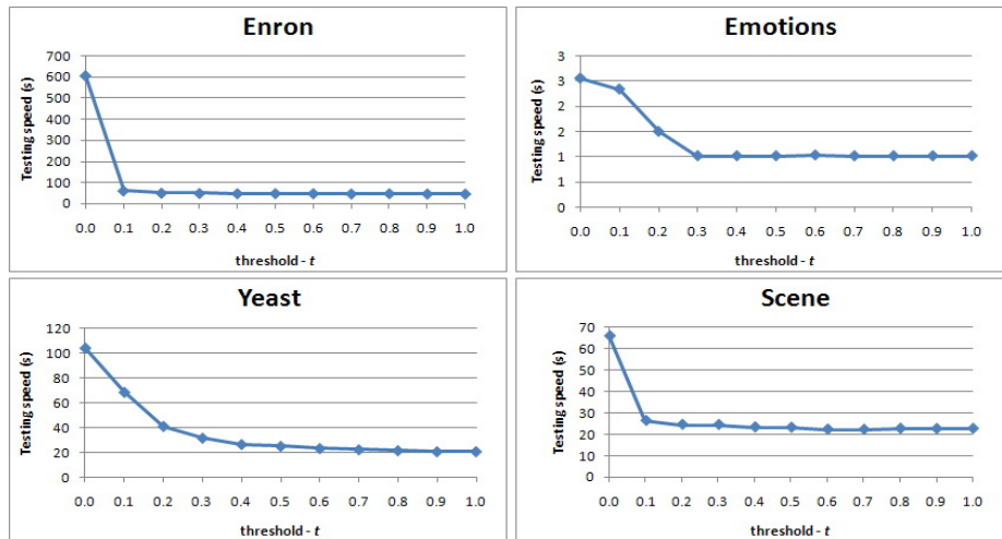
Fig. 3. Testing time of TSVA as a function of the threshold t ( 0 \leq t \leq 1 ) for each dataset measured in seconds
