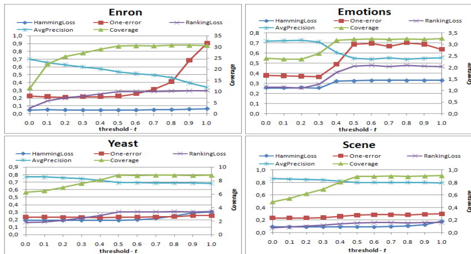
Fig. 2. Predictive performance of TSVA as a function of the threshold t ( 0 \leq t \leq 1 ) for each dataset
